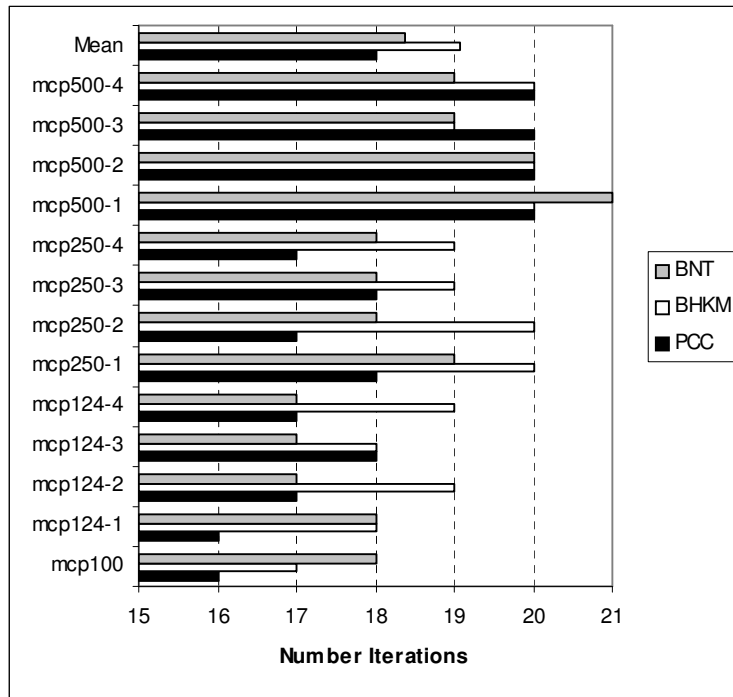
Figure 13: Number of iterations for the mcp class.
